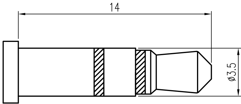
MATING PLUG
