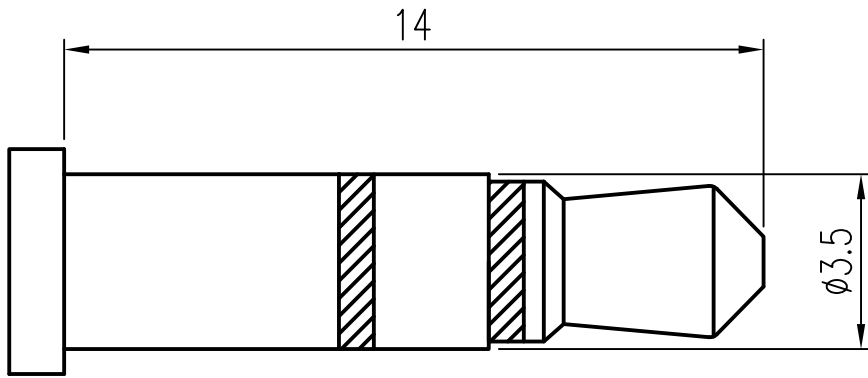
MATING PLUG
