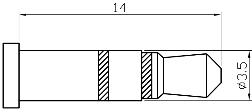
MATING PLUG
