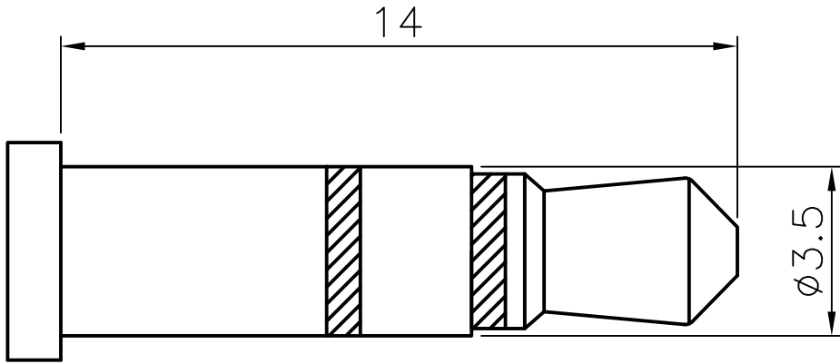
MATING PLUG
