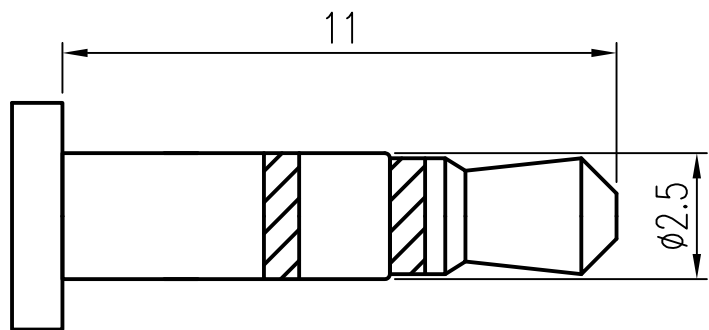
MATING PLUG
