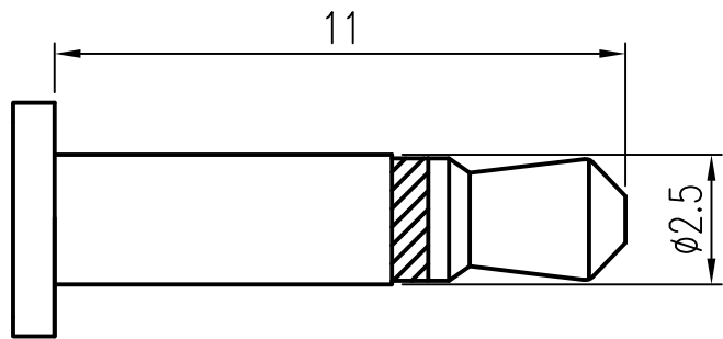
MATING PLUG
