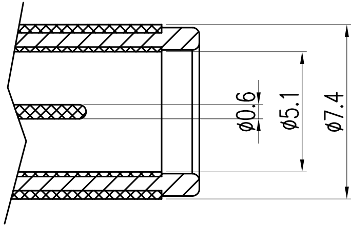
MATING PLUG
