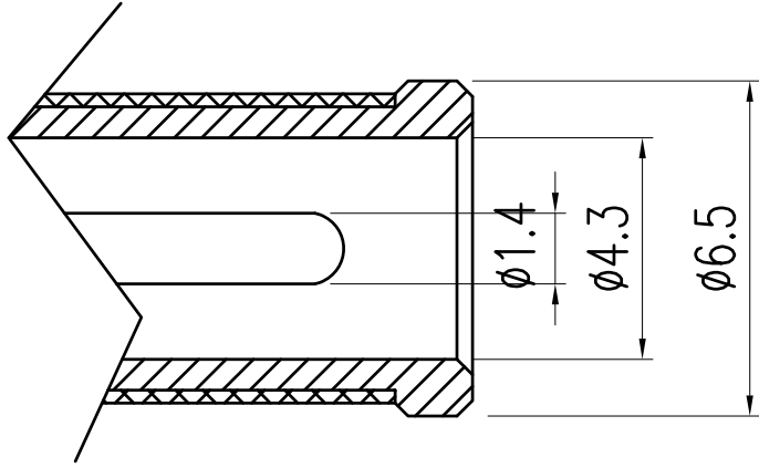
MATING PLUG
