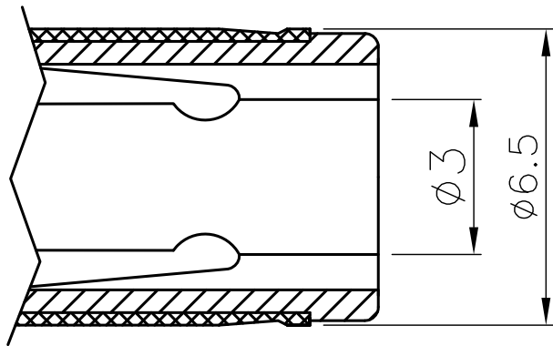
MATING PLUG
