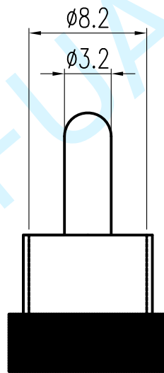
MATING PLUG
