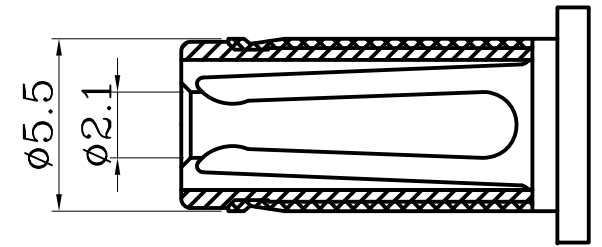
MATING PLUG
