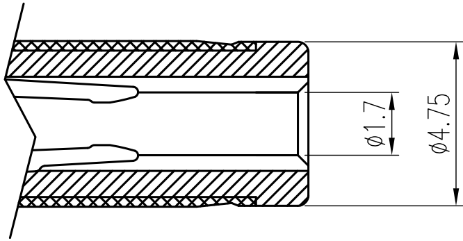
MATING PLUG
