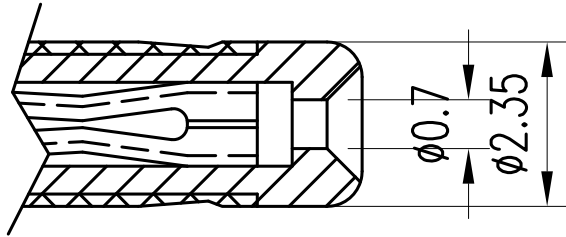
MATING PLUG
