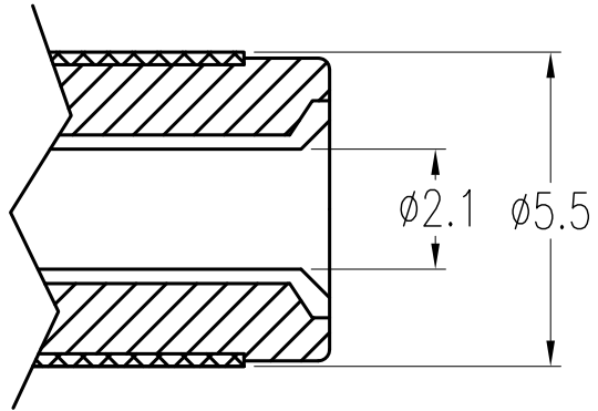
MATING PLUG
