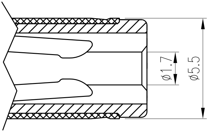
MATING PLUG
