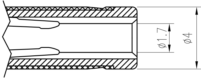
MATING PLUG
