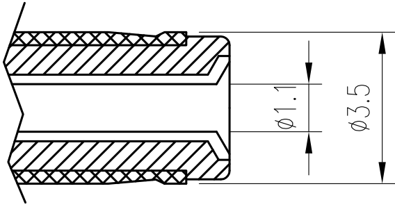
MATING PLUG
