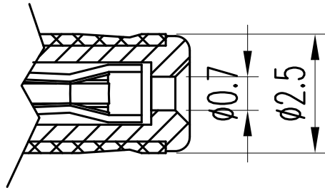
MATING PLUG
