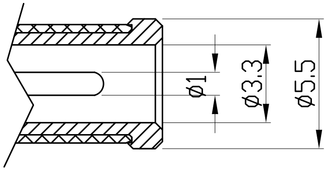
MATING PLUG
