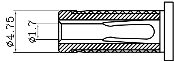
MATING PLUG
