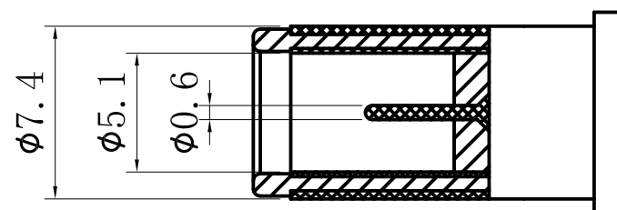
MATING PLUG
