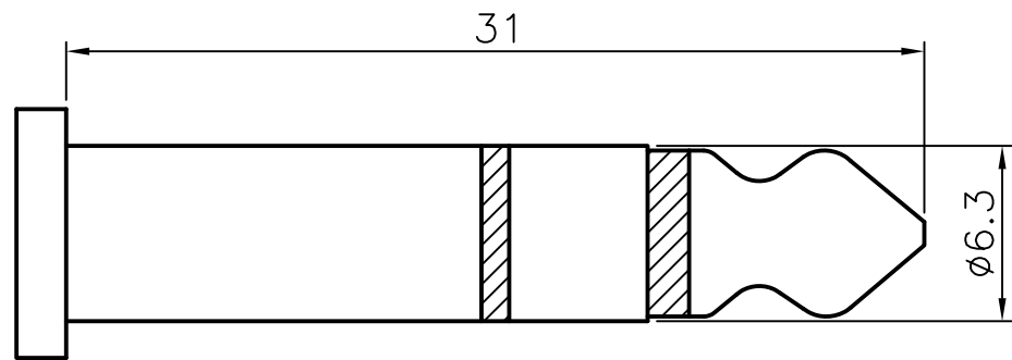
MATING PLUG
