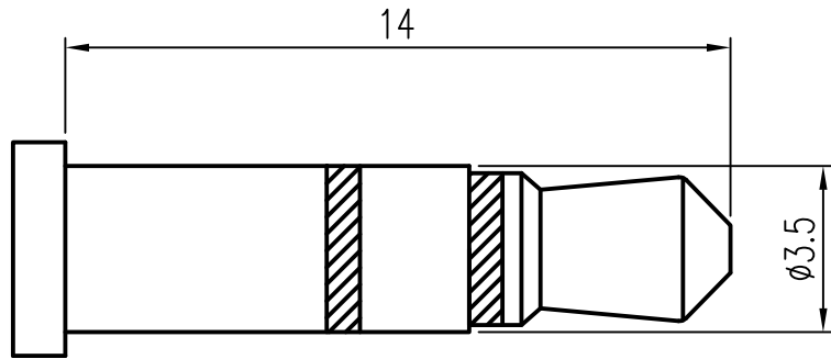
MATING PLUG
