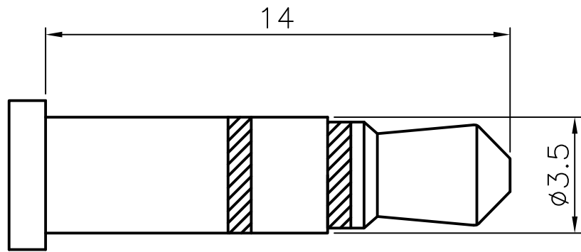
MATING PLUG
