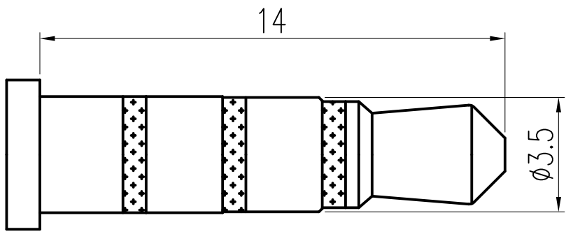
MATING PLUG
