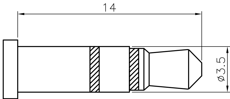
MATING PLUG
