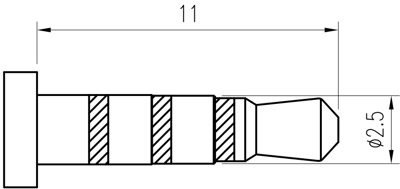
MATING PLUG
