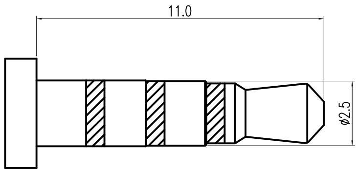
MATING PLUG
