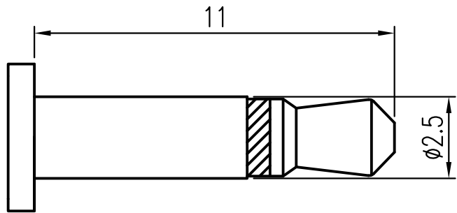
MATING PLUG
