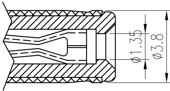
MATING PLUG
