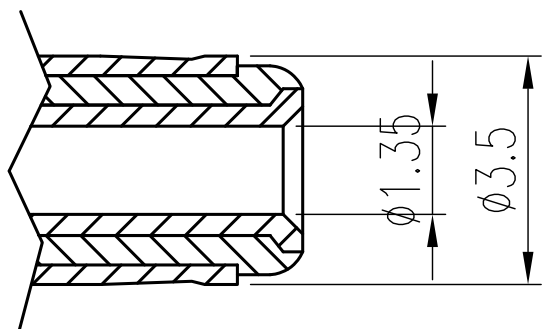
MATING PLUG
