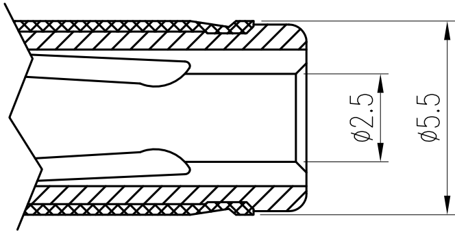
MATING PLUG
