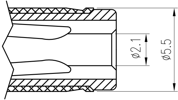
MATING PLUG
