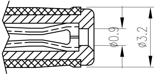
MATING PLUG
