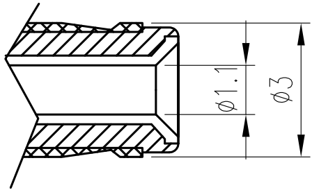
MATING PLUG
