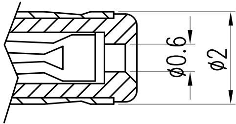
MATING PLUG
