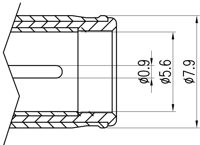
MATING PLUG
