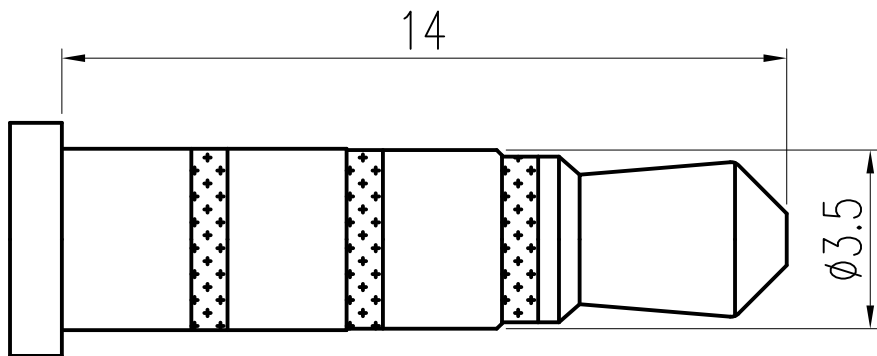
MATING PLUG
