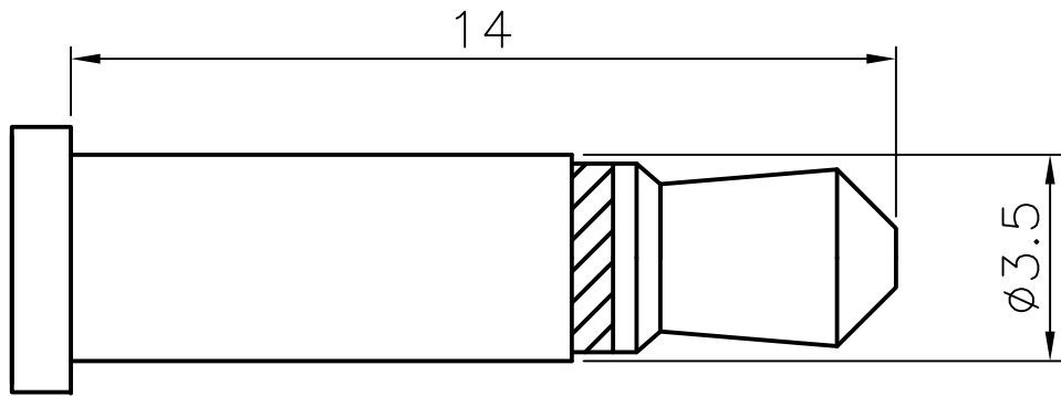
MATING PLUG
